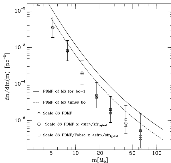
Fig. 1. Corrections to Scalo (1986) PDMF; see text.
