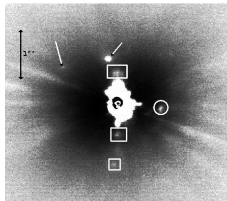
Fig. 1. Residuals from one of our targets after of the PSF subtraction. Some residuals correspond to real objects (arrows); others are due to optical effects or imperfect fitting of the PSF model (circles, squares).
