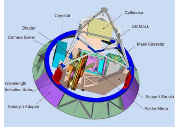
Fig. 2. OSIRIS optomechanical layout. The different subsystems are indicated. Some parts have been removed to provide a clearer view.
