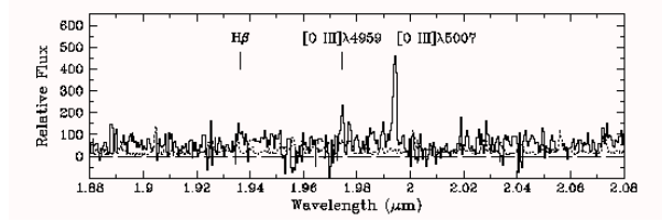
Fig. 2. NIR K band spectrum of a Lyman break galaxy ( z = 2.979 ) showing H\beta , [[O\ III] 5007\text{\AA}] and the stellar continuum. The dotted line is the 1\sigma error spectrum. From Pettini et al. (2001).
