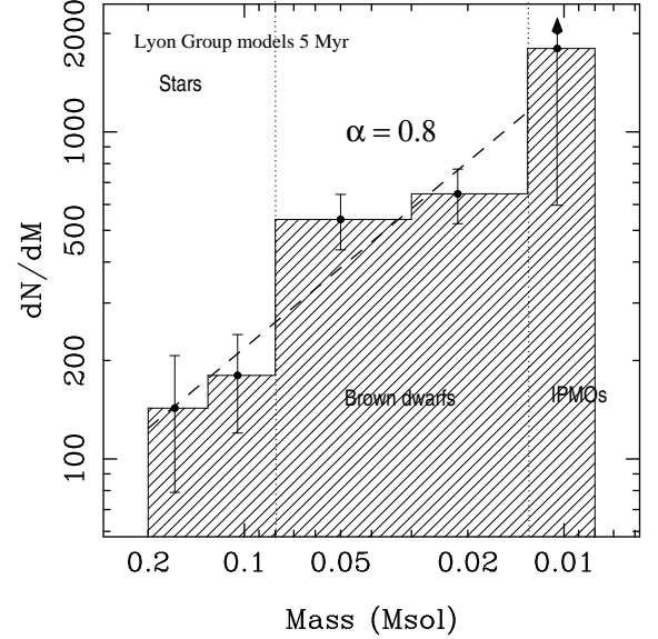
Fig. 1. Substellar mass function in the young star cluster \sigma Orionis, adapted from Béjar et al. (2001).
