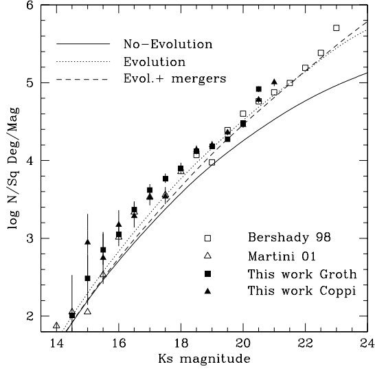
Fig. 2. Groth strip and Coppi field galaxy number counts. Number counts in K band from Bershadly et al. (1998) and Martini (2001) are shown for comparison. Predictions for galaxy number counts were obtained with ncmod (Gardner 1998) using the q_0 = 0.02 , H_0 = 50 \text{ km s}^{-1} \text{ Mpc}^{-1} cosmology.
