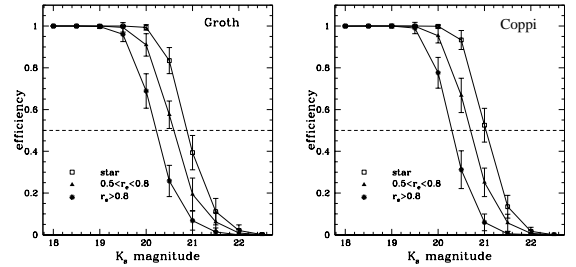
Fig. 1. Detection efficiencies for the Groth (left panel) and Coppi (right panel) fields, estimated using real object as models. Points and error bars are for 30 simulations for each 30 objects of the same size class and magnitude.
