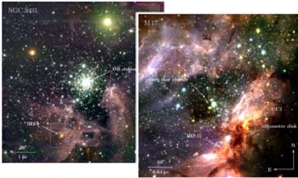
Fig. 1. ISAAC JHK s data of NGC 3603 (left) and M17 (right). Dashed boxes outline the position of the NGC 3603 IRS 9 sources (shown in Figure 2) and of the discussed M17 sources (IRS 15, UC 1 and silhouette disk; see Figure 3).
