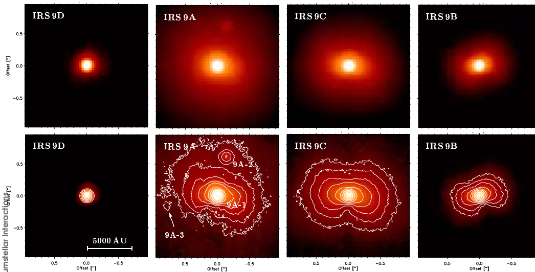
Fig. 2. NACO L' data of the protostellar candidates NGC 3603 IRS 9A, IRS 9B and IRS 9C, in contrast to the PSF reference source NGC 3603 IRS 9D.
