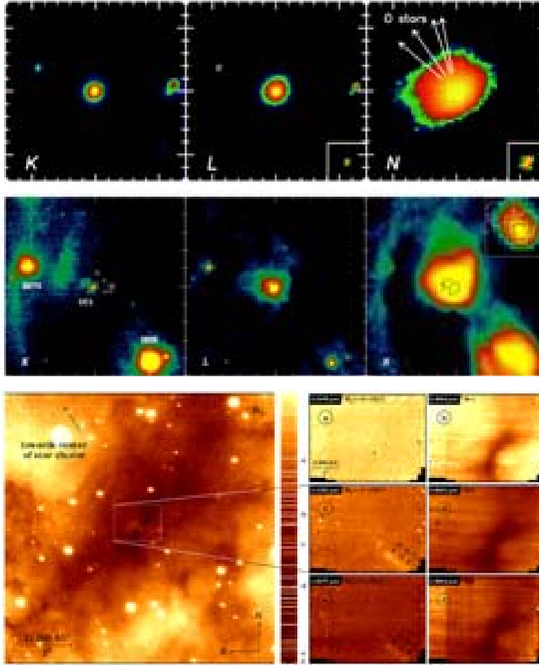
Fig. 3. Top row: ISAAC K s and L' data together with VISIR N data of the ZAMS source M17 IRS 15. Middle row: NACO K s and L' data as well as VISIR N data of the HC H II candidate M17 UC 1. Bottom row: NACO K s image (left) and SINFONI integral field spectroscopy (right) of the M17 silhouette disk and associated H 2 jet.
