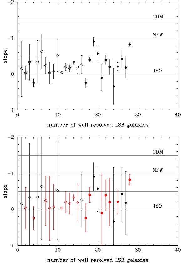
Fig. 1. Top: Plots of the slopes for the 16 best resolved galaxies of the De Blok et al. (2001b) sample (open circles) and the additional 12 galaxies in the De Blok & Bosma (2002) sample (filled circles), with 1\sigma error bars; Bottom: Same, but with 3\sigma error bars. 17 points are 3\sigma away from the NFW prediction.
