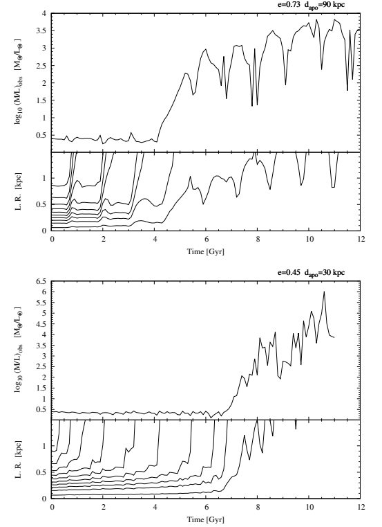
Fig. 2. Mass-to-light ratios for satellites with initial mass of 10^7 M_{\odot} (top) and 10^8 M_{\odot} (bottom). For both satellites the Lagrange radii, as in Figure 1, have been included to locate start of disrupted phase.
