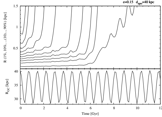
Fig. 1. Lagrange radii containing (bottom to top) 1%, 10%, 20%, ..., 90% of the initial mass of a satellite with 10^7 M_{\odot} . Bottom panel: galactocentric distance of the density maximum. The parameters of the orbit are given in the upper right corner.
