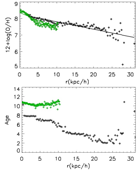
Fig. 1. Upper panel: Stellar abundance gradients for the disc (black symbols) and central spheroid (green symbols) components. The continuous line: linear fit; lower panel: Mean age of the disc (black) and central spheroid (green) components.
