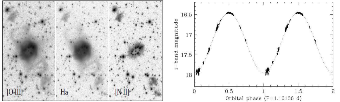
Fig. 1. Left: Narrow band [OIII], H \alpha and [NII] images of IPHASX J194359.5+170901 taken with the NOT Telescope (ORM, La Palma) with a field of view of 70 \times 110 arcsec 2 . North is up and East is left. Right: Light curve of the central star indicating a binary system with a period of \sim 1.16 days (Corradi et al. 2011).
