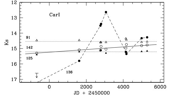
Fig. 2. Light curves in the K_s band, from 1993 November to 2010 April, of the young variable embedded stars (Tapia et al. 2006) Car I #136 (filled circles) and #125 (open circles). The photometric data of the comparison (non-variable) stars #91 (open triangles) and #142 (filled triangles) in the same field are also plotted.
