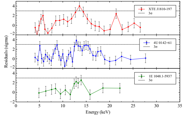
Fig. 1. Observed emission line spectrum from three different AXP sources: XTE J1810-197, 4U 0142+61 and 1E 1048.1-5937 (Burst 3). These spectra represent the residuals after subtraction of the best fit continuum. All show a strong, significant feature at \sim 13 keV. Data from Gavriil et al. (2011). The color figure can be viewed online.
