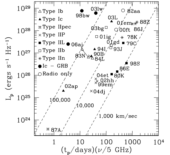
Fig. 1. Peak luminosity and corresponding epoch for the well-observed radio supernovae. The dashed lines give curves of constant expansion velocity, assuming synchrotron self-absorption at early times (updated version of Figure 4 in Chevalier 1998).
