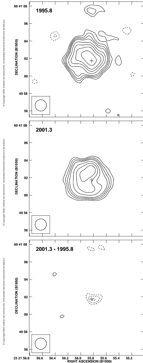
Fig. 1. Continuum images of KJPN 8 for 1995.8 (top) and 2001.3 (center), with contours of -4 , -3 , 3 , 4 , 5 , 6 , 8 , 10 , 12 , and 15 times 10 \mu\text{Jy beam}^{-1} , the average rms noise of the two maps. At the bottom we show the difference image (2001.3 - 1995.8), with contours of -5 , -4 , -3 , 3 , 4 , and 5 times 14 \mu\text{Jy beam}^{-1} , the rms noise of the map. The cross marks the position of the stellar nucleus.
