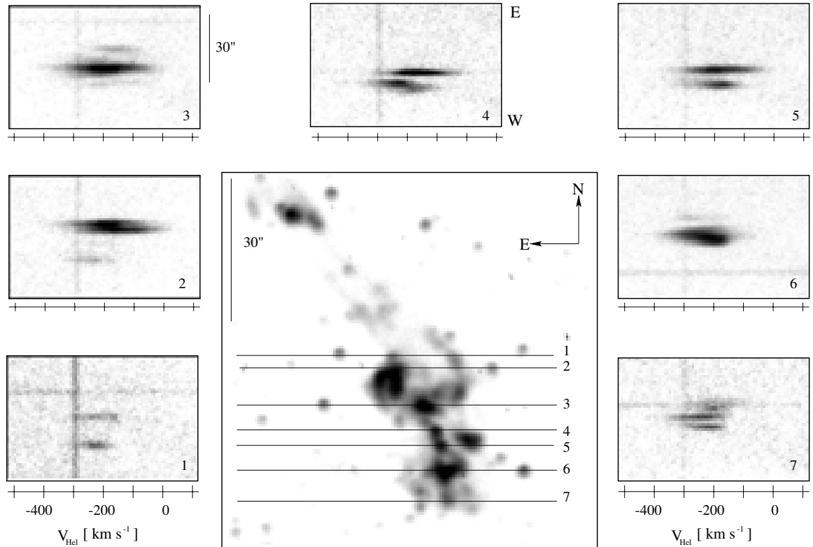
Fig. 3. Set of seven long-slit echelle spectra obtained across H 2-12. Slit positions are indicated over a logarithmic H\alpha image. All slits are oriented E-W. The [N\text{ II}] \lambda_c 6585 \text{ \AA} line profiles extracted from these slit positions are shown as position-velocity diagrams.
