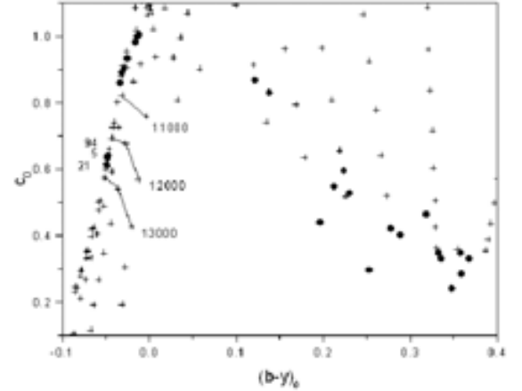
Fig. 6. Location of the stars of the farthest cluster in the grids of LGK86 for solar composition. The hottest stars have been indicated by their Webda numbers. The other numbers represent the temperature in K.
