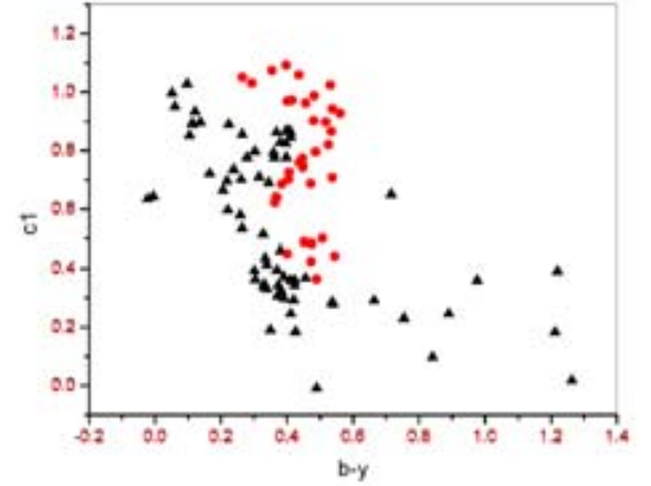
Fig. 2. Location of the measured stars in the (b-y) vs c_1 diagram. The whole sample is separated into two discernible groups and marked by triangles and dots.
