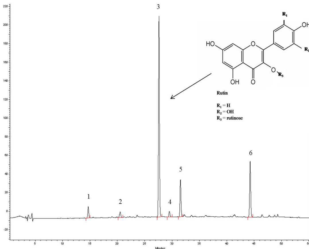
Figure 1 Typical chromatogram of E. suberosum extract.
