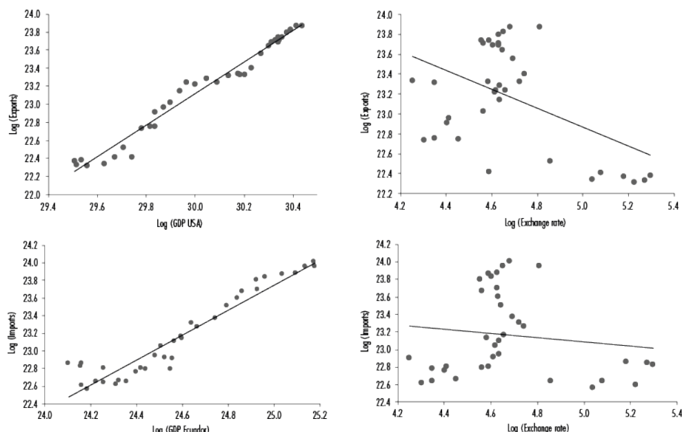
Figure 3. Correlation between the logs of the variables
