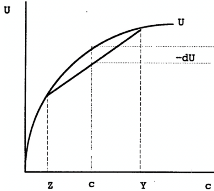
Figure 2. Graph – positive, increasing, concave utility function
