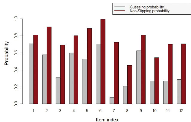
Figure 1. Parameters for the DINA model
