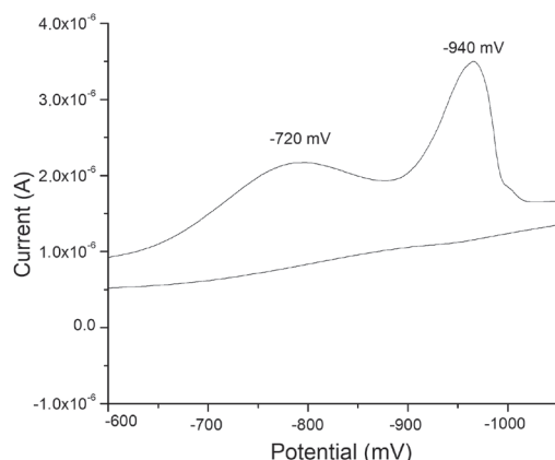
Figure 1. Sweep polarograms of chlorpyrifos. Standard of CP for the potential of electroactivity, the analyte had two signals: -720 and -940 mV. The second polarogram corresponds to blank.
