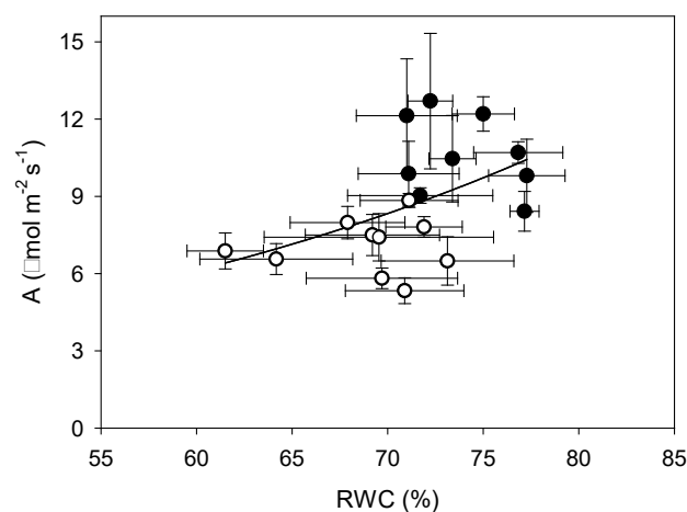
Figure 2. Relationships between \text{CO}_2 assimilation rate and relative water content in ten Ecuadorian cacao clones, during dry (open circles) and rainy seasons (closed circles). The regression including both seasons all clones is represented by the solid line; r^2 = 0.30 .
