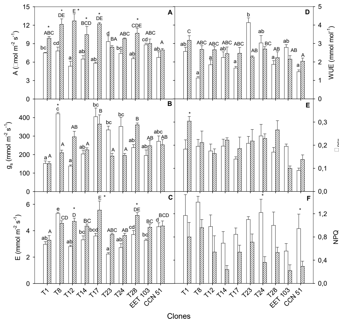
Figure 1. A, \text{CO}_2 assimilation rate; B, stomatal conductance; C, transpiration rate; D, water use efficiency; E, relative quantum yield of PSII; F, non-photochemical quenching coefficient in Ecuadorian cacao clones measured during the dry (open bars), and the rainy (striped-bars) seasons. Different small letters represent significance between clones during DS; different capital letters represent significance between clones during RS. Asterisks (*) represent a significant difference between dry and rainy season conditions for the same clone.
