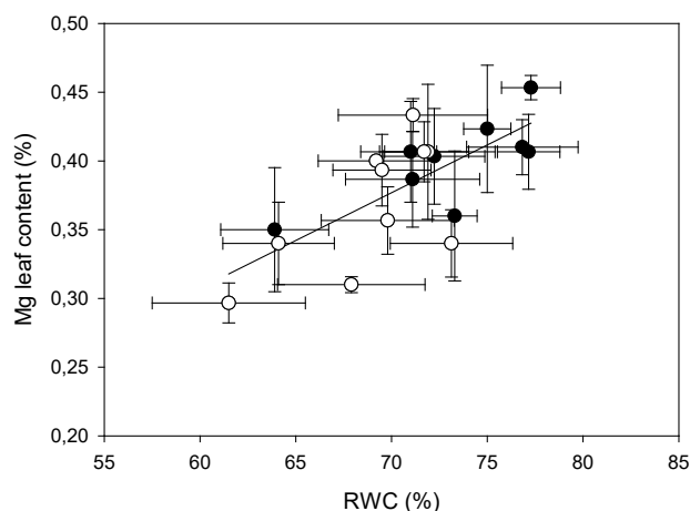
Figure 3. Relationships between leaf Mg content and relative leaf water content in ten Ecuadorian cacao clones during dry (open circles) and rainy seasons (closed circles). The regression including both seasons all clones is represented by the solid line, [Mg] = 0.0069 \times RWC - 0.1093 ; r^2 = 0.52 .
