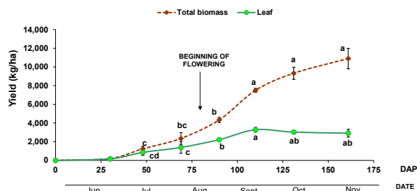
Figure 2. Biomass accumulation and partitioning during the vegetative stage in 2014. PD was not considered due to the lack of significant differences; average values are represented. Vertical bars represent standard error of the mean ( \pm ). Different letters mean significant statistically difference for P < 0.05 .
