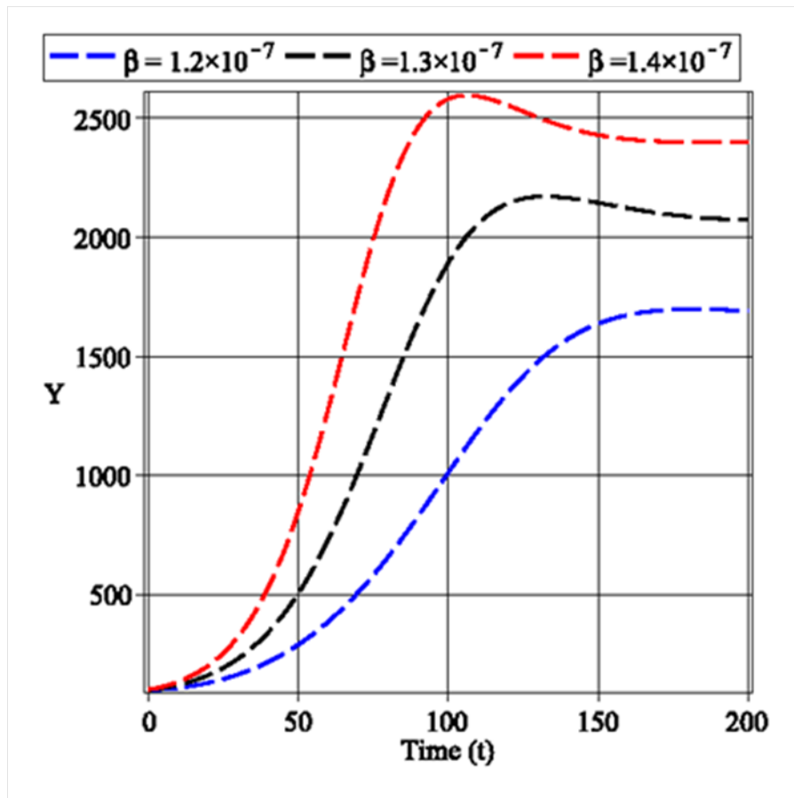
FIG.4: Infected population density ( Y) Vs. time ( t) in days for various values of constant contact rate (B).
