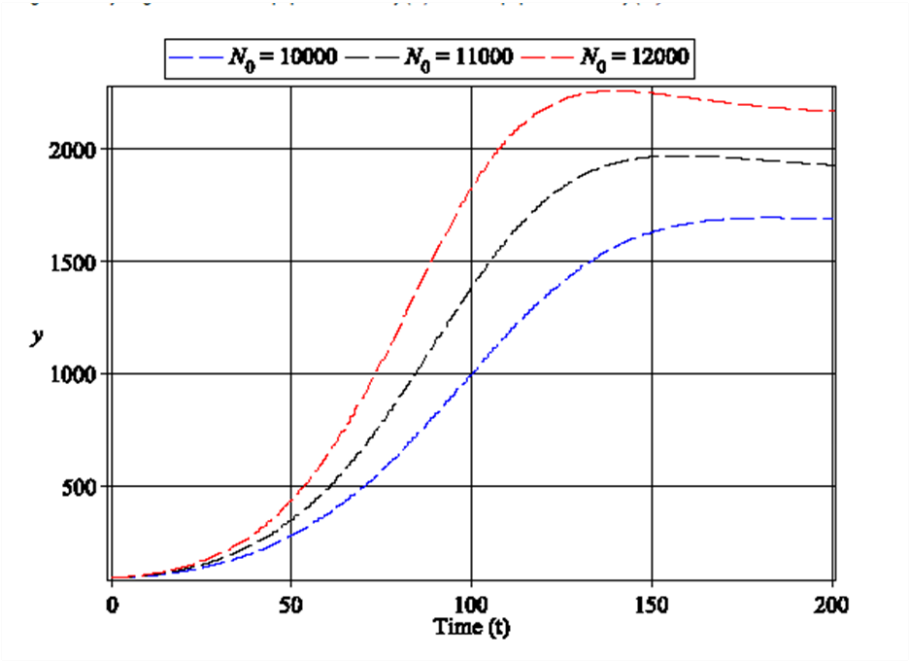
FIG.2: Infected population density ( Y ) Vs. time ( t ) in days for various values of non-emigrating population density ( N_0 ).
