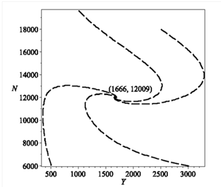
FIG.1. Stability diagram for infective population density ( N ) and total population density
