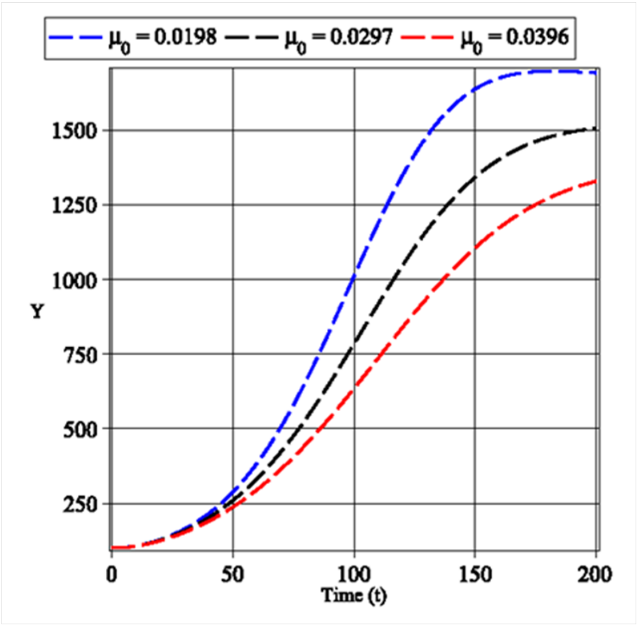
FIG.5: Infected population density (Y ) Vs. time ( \tau ) in days for various values of variable emigration rate ( M_0 )
