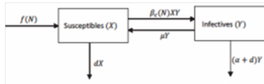
FIG 1. Schematic flow of the Disease
