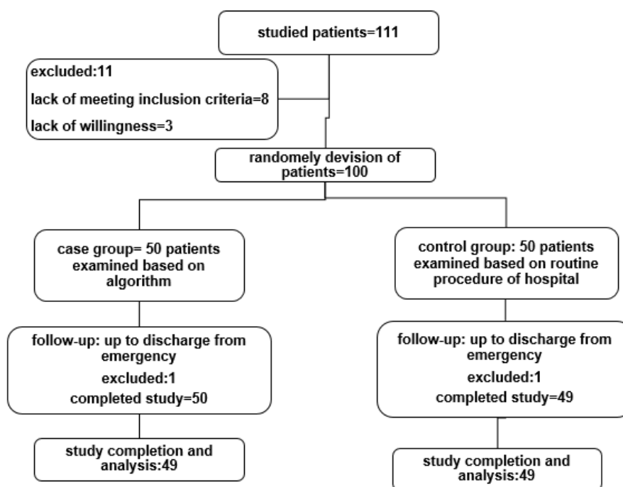
FIGURE 2. Study flowchart
