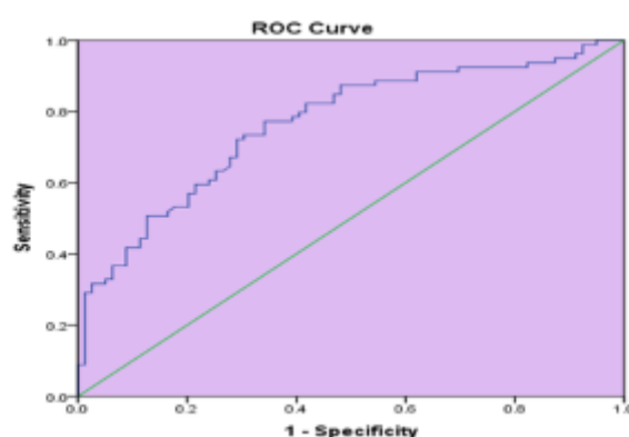
FIG 4: Roc curve for sensitivity and specificity cutoff point of N/L ratio. Area Under the Curve 0.76, N/L ratio (2.7) with sensitivity 76% and specificity 66%
