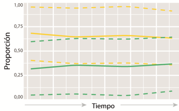
B787 ( M_1 )
