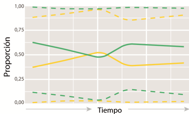
PDEM1 ( M_3 )
