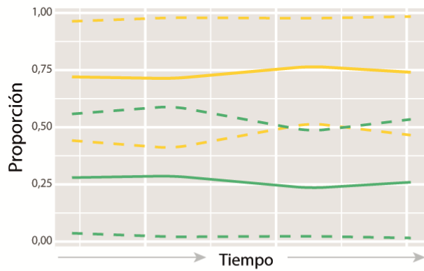
CT19 ( M_2 )
