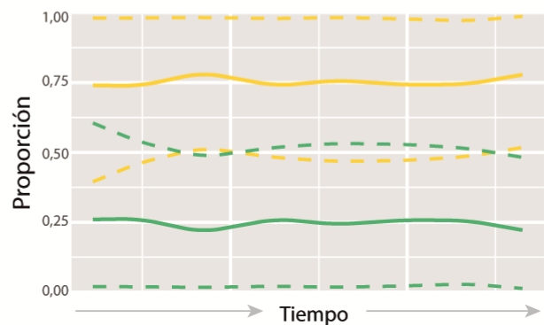
PDEM2 ( M_3 )
