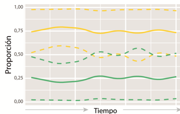
B816 ( M^2 )
