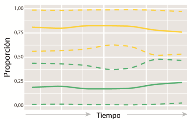
PDEM1 ( M_3 )
