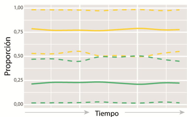
PDEM2 ( M_3 )
