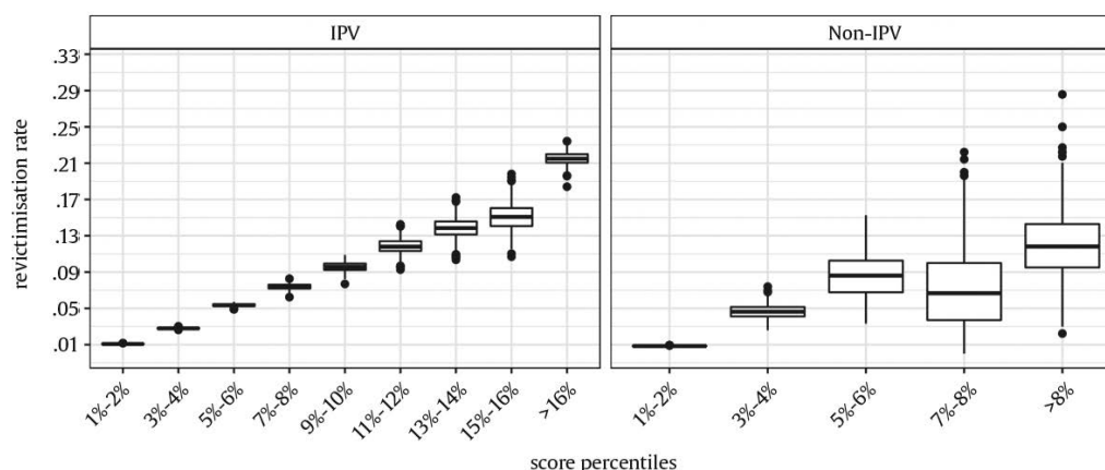
Figure 3. Model Calibration on Full Variable Set.
