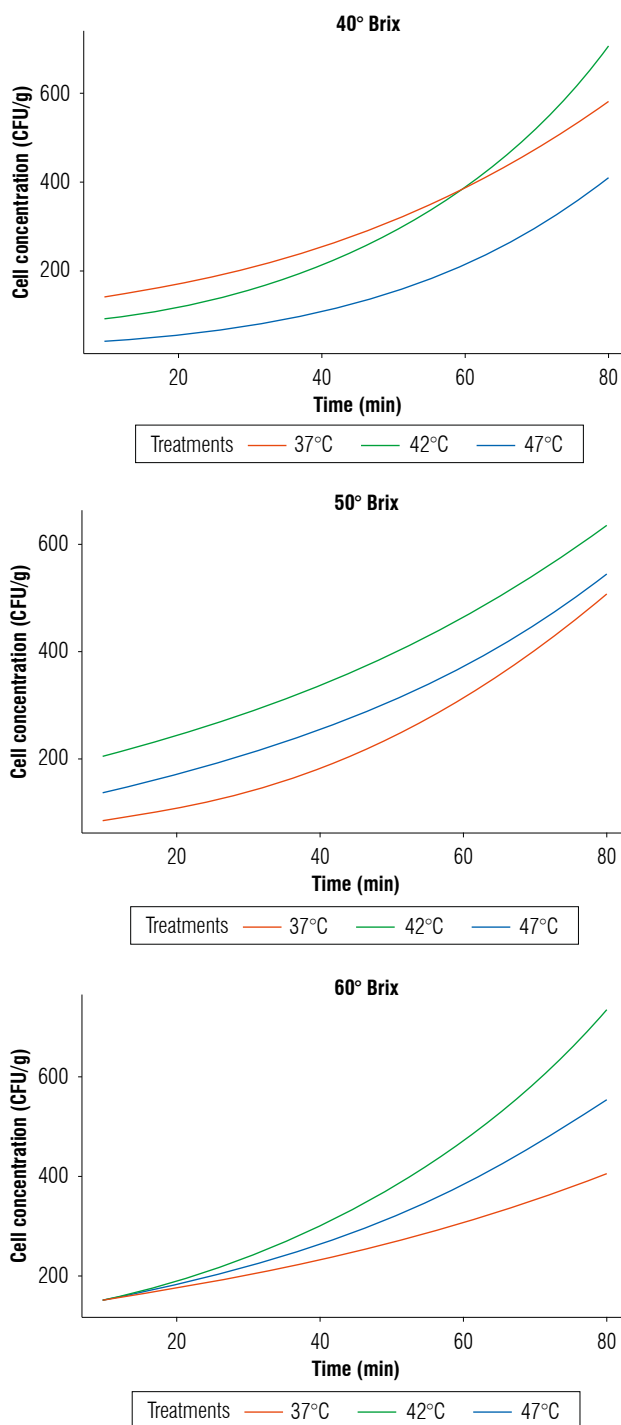
FIGURE 3. Microbiological kinetics of Saccharomyces boulardii in apple cubes at different concentrations of solids and temperatures.
