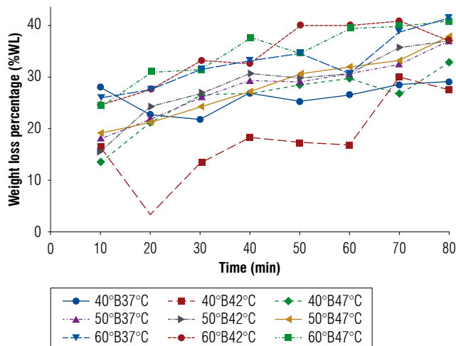
FIGURE 1. Weight loss percentage (%WL) as a function of time of apple cubes inoculated with Saccharomyces boulardii at different concentrations and temperatures.
