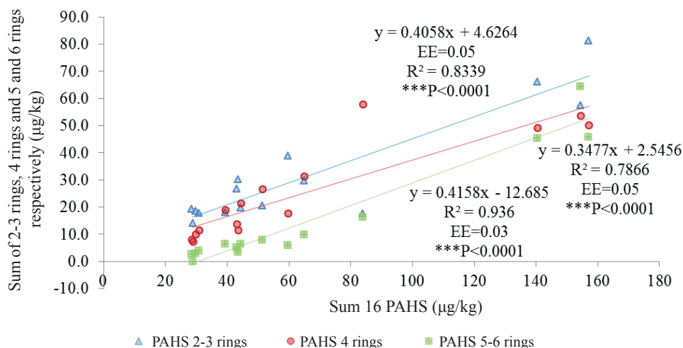
Figure 2. Performance of polycyclic aromatic hydrocarbons (PAHs) in the grass vs. the sum of PAHs of 2-3; 4; 5-6 rings.
