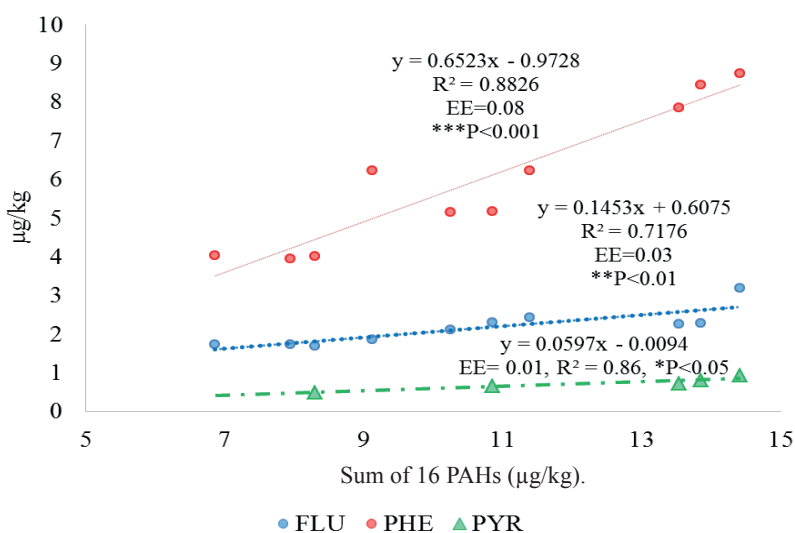
Figure 6. Concentration of FLU, PHE and PYR (µg/kg) vs. sum of 16 PAHs (µg/kg).
