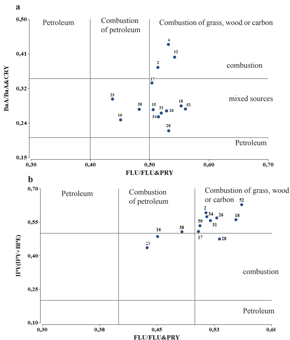
Figure 4. Relations of the polycyclic aromatic hydrocarbons (PAHs) that indicate possible origins of the contamination in the grasses. (a) BaA / (BaA + CHRY) vs FLU/(FLU + PRY); (b) IPY / (IPY + BPE).
