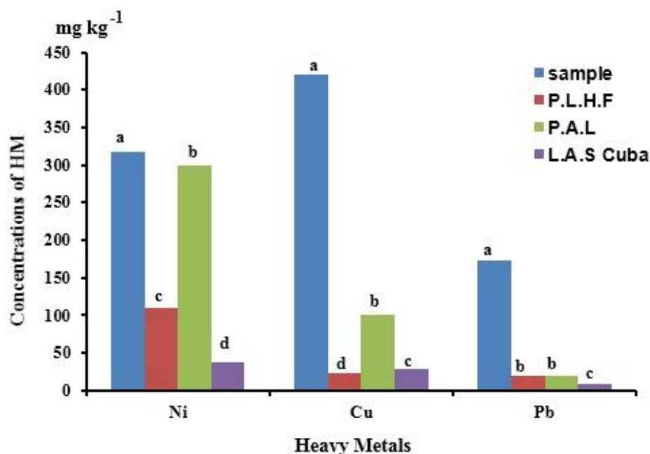
Figure 2. Concentration of Ni, Cu and Pb compared to average levels acceptable for healthy food production and phytotoxic levels
