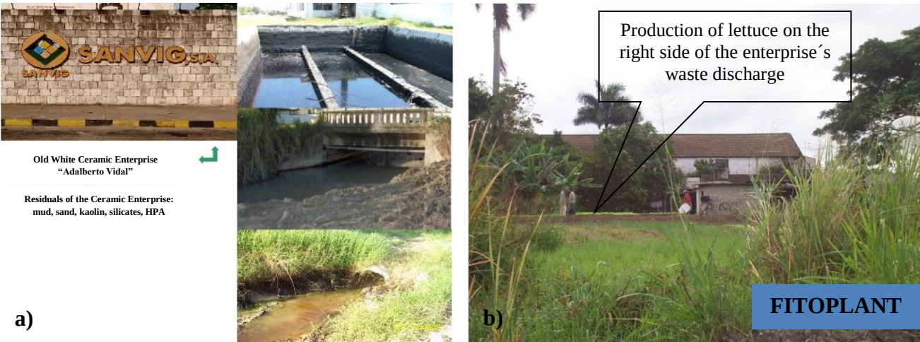
Figure 1. a) Expulsion and transit of the Enterprise's residuals b) Production area
