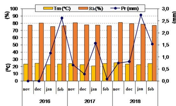
Figure 1. Behavior of meteorological variables in the periods from November to February 2016 to 2018. Monthly mean temperature (Tm), Monthly relative humidity (Hr), Monthly mean precipitation (Pr)
