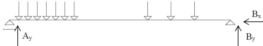
Figure 4: Outline of an isostatic beam with three unknowns.
