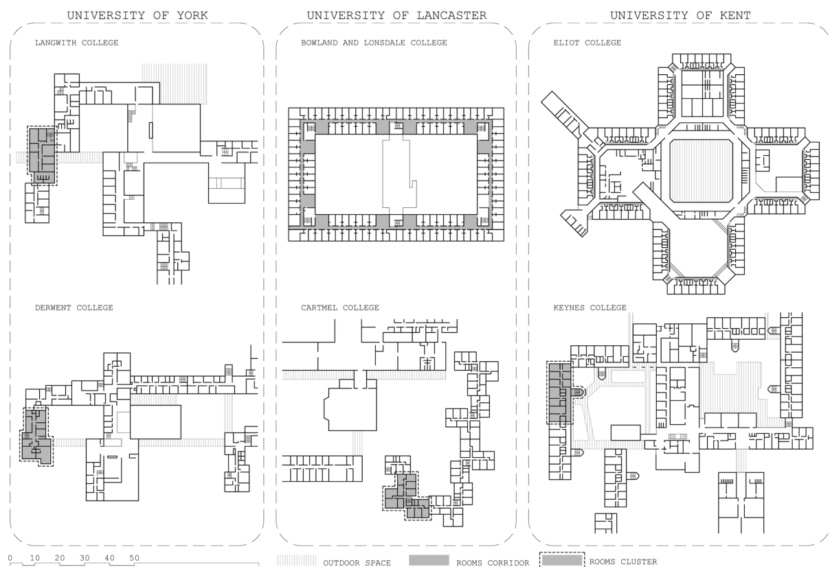
Figure 4: Layout strategies for colleges.
