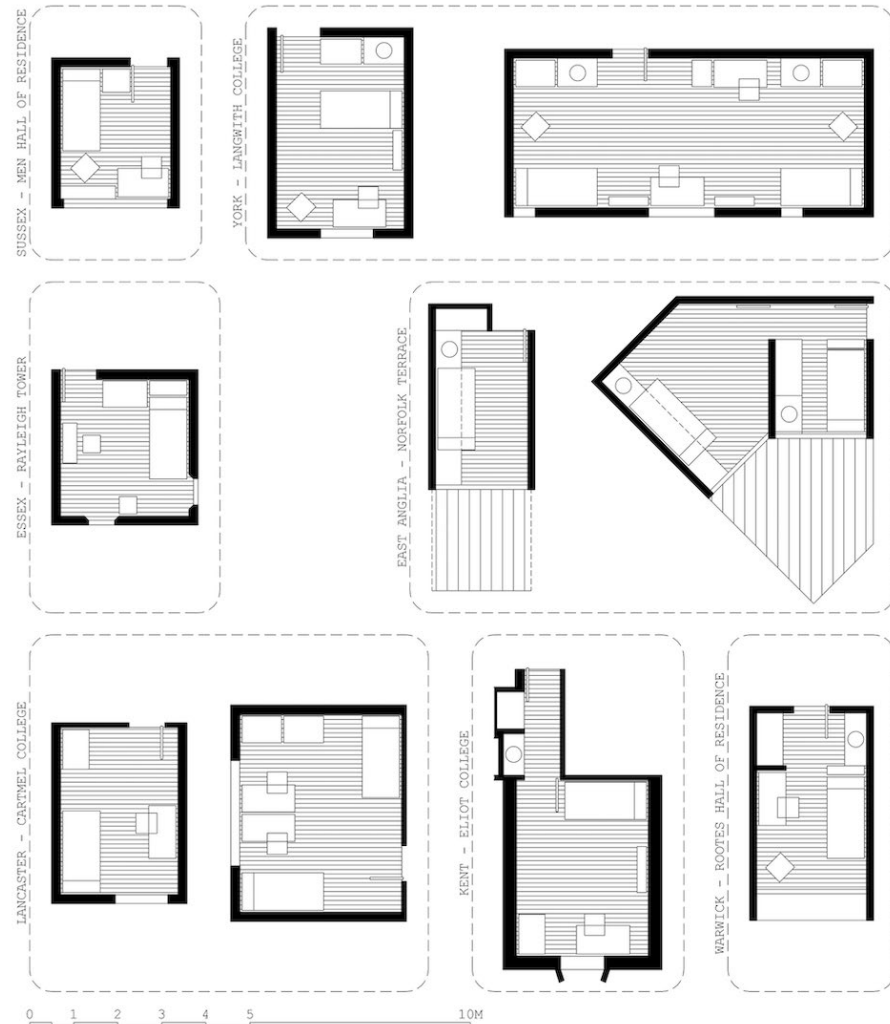
Figure 6: Analysis of bedrooms at plateglass universities.
