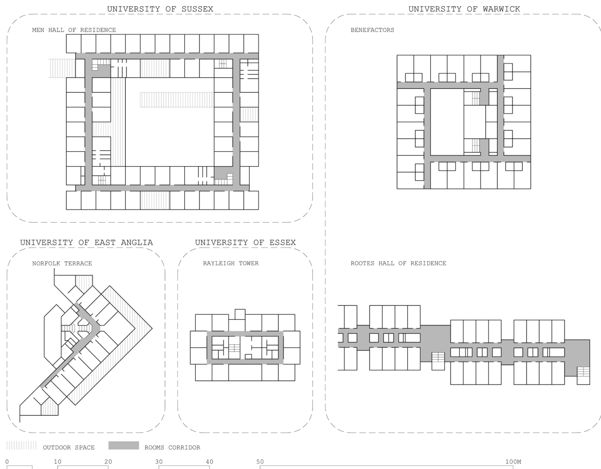
Figure 5: Layout strategies for halls of residence.
