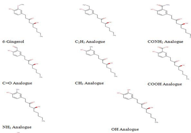
Fig. 3. The two dimensional (2D) structure of 6-gingerol and its modified derivatives as designed using the MarvinSketch software.
