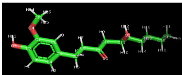
Fig. 4. 3D structure of 6-Gingerol showing all labeled atoms.
