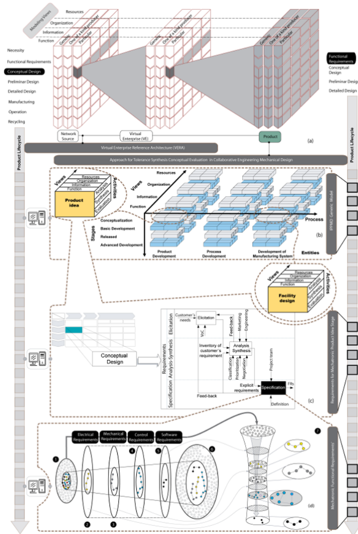
Fig. 1 Mechatronic product design requirements decomposition
