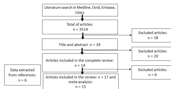
Figure 1 Search Flowchart
