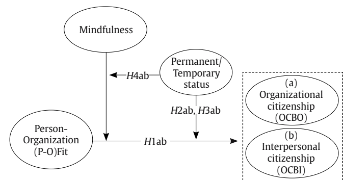
Figure 1. Hypothesized Model.
