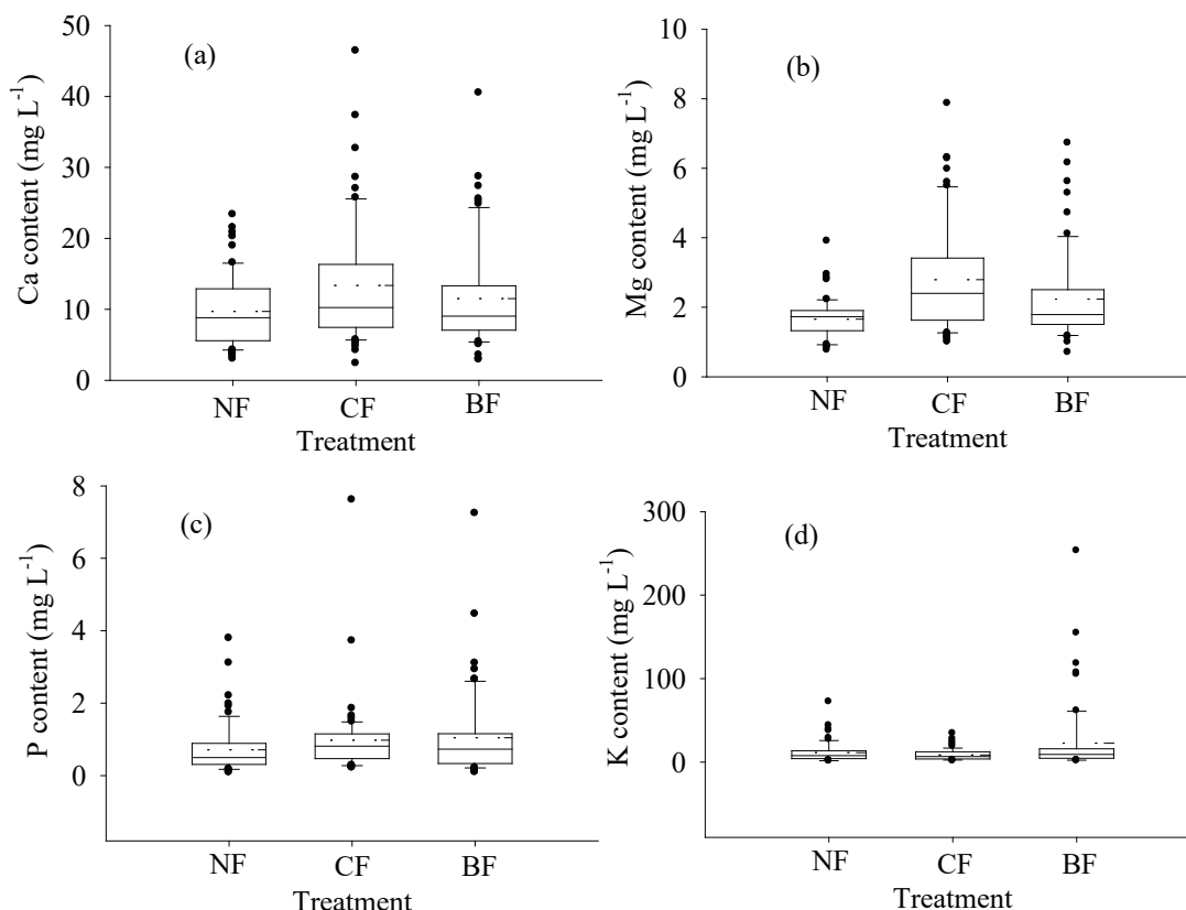
Figure 1. Calcium (Ca; a), magnesium (Mg; b), phosphorus (P; c) and potassium (K; d) contents in the runoff water. NF: native field; CF: cultivated field; BF: burned field, for an Inceptisol.
