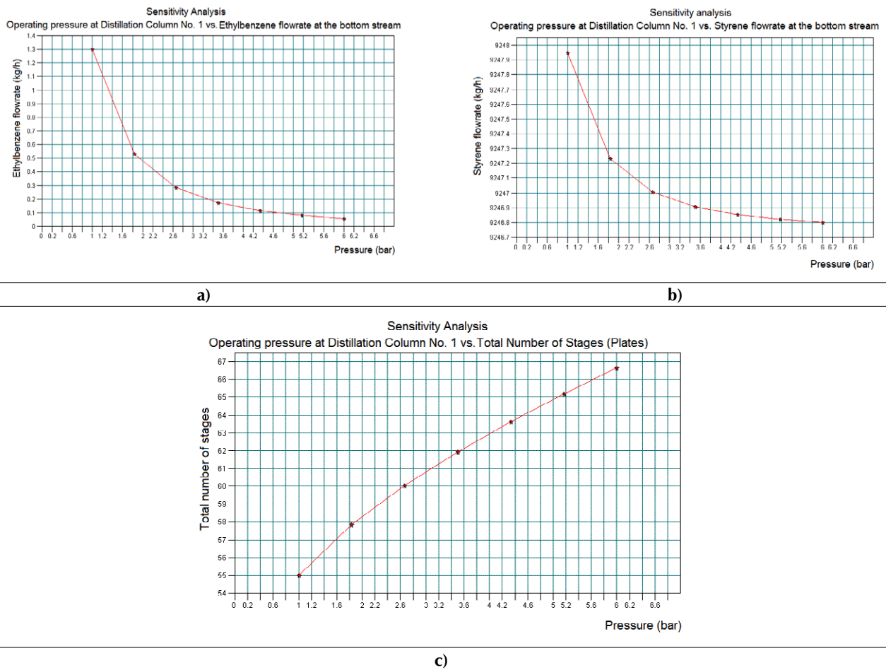
Figure 6. Results obtained in the Sensitivity Study No. 2 by means of CHEMCAD® simulator
