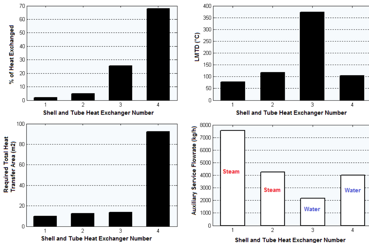
Figure 3. Results obtained for the shell and tube heat exchangers
