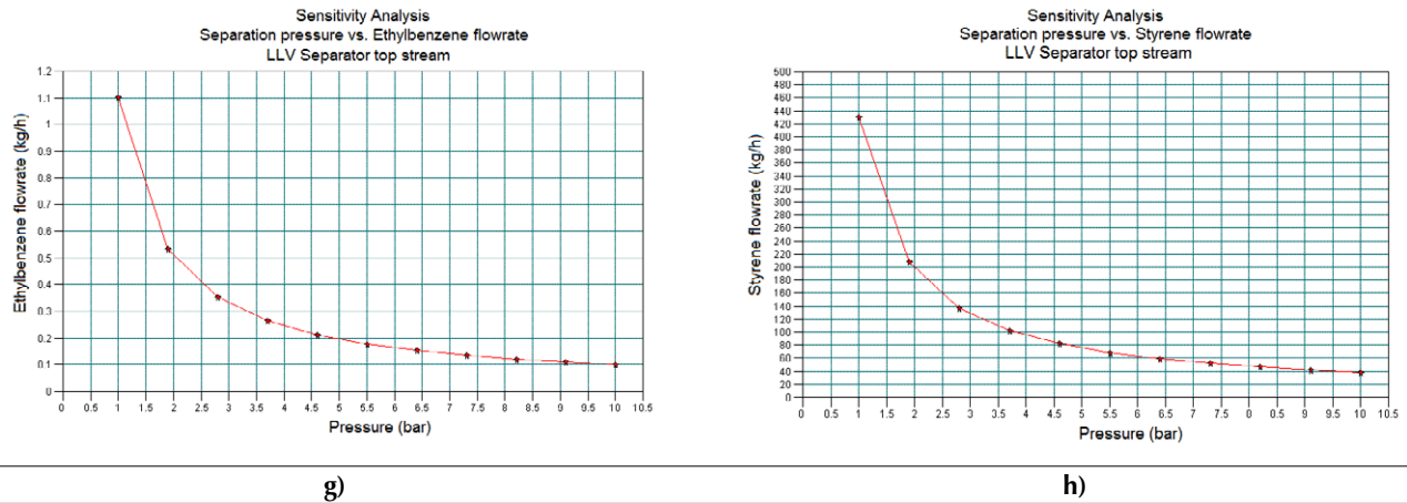
Figure 5. Results obtained in the Sensitivity Study No. 1 by means of CHEMCAD® simulator
