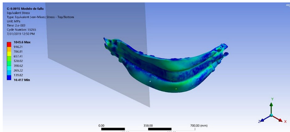
Figure 11. Von Mises results at 56 Km/h
