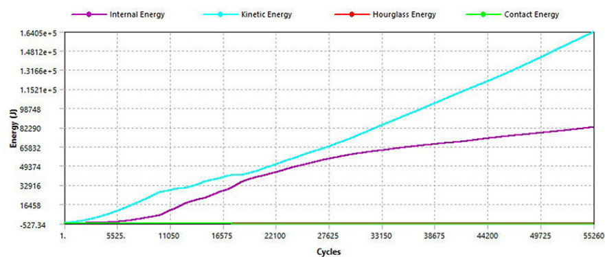
Figure 12. Energy results at 56 Km/h
