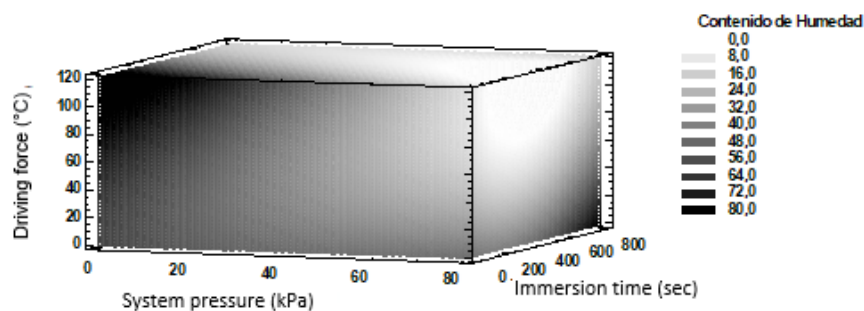
Figure 3. Color change response surface 3d mesh chart in apple snack Source: Own elaboration
