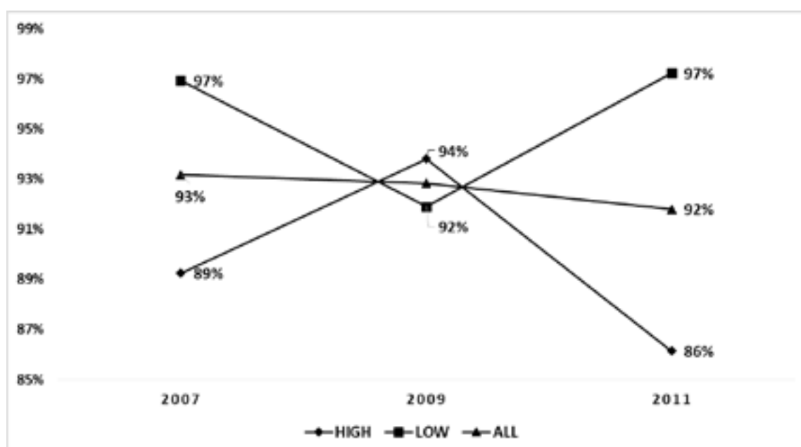
Figure 4 - Average Efficiency (BCC-INPUT) as a function of per capita expenditure
