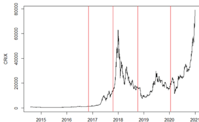
Figure 1 - Period Division by CRIX Quotations
