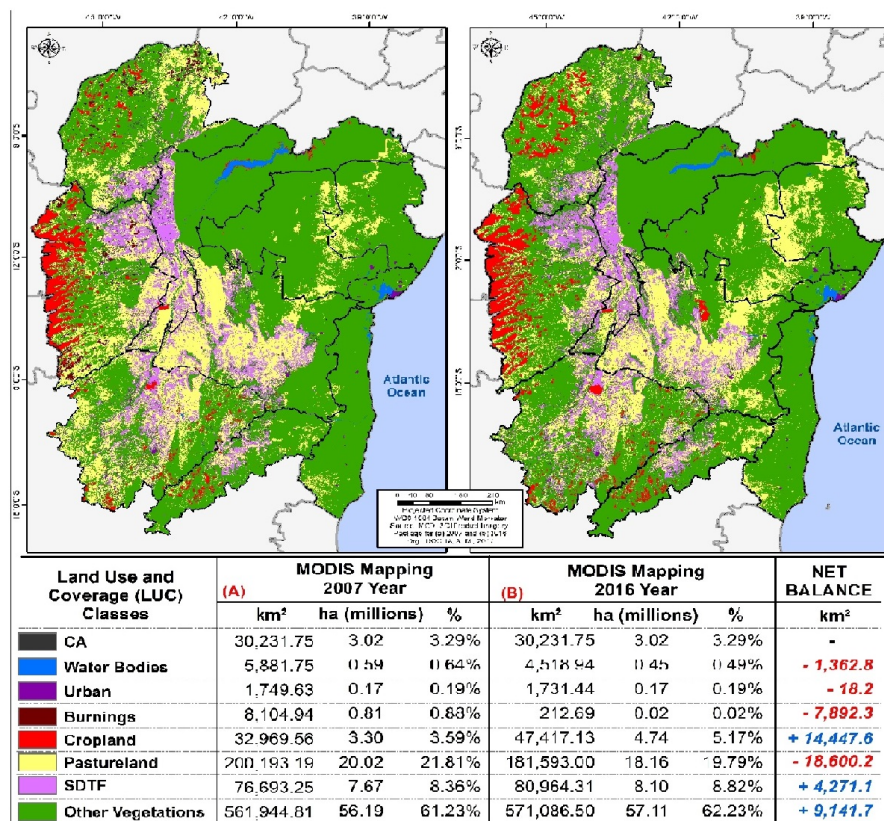
FIGURE 5 Distribution of Land Use and Coverage Classes and associated Statistics for the Years 2007(A) and 2016 (B)
