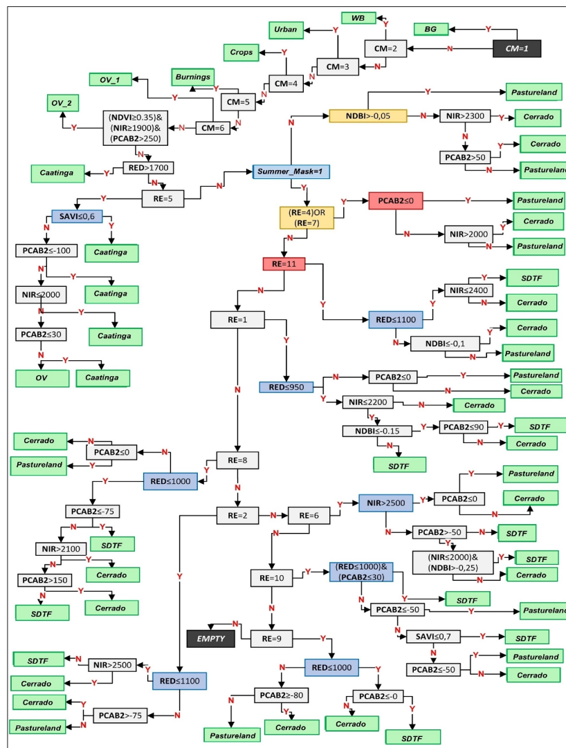
FIGURE 3 Decision Tree for 2016 MODIS Classification
