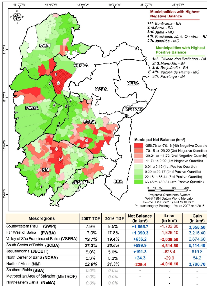
FIGURE 6 Municipal Distribution of the Net Balance (Loss and Gain) of Seasonally Dry Tropical Forest and statistical summary (% Distribution SDTF, Net Balance, Gain and Loss) of the Mesoregions of the Study Area.
