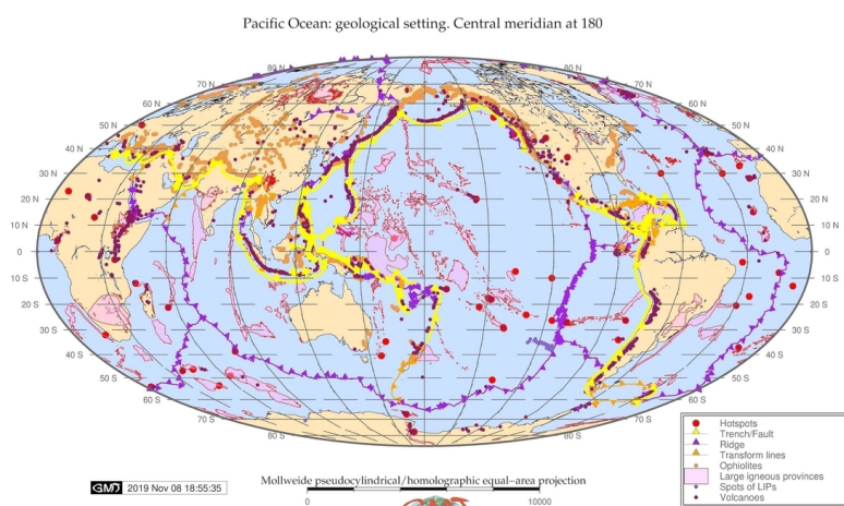
FIGURE 2 Geologic map of the Pacific Ocean region. author
