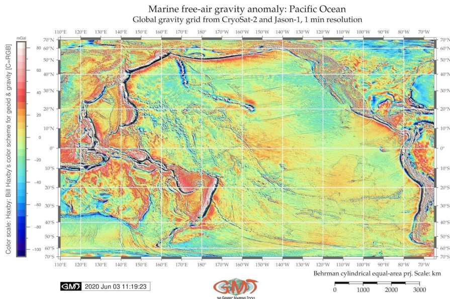
FIGURE 5 Marine free-air gravity anomalies of the Pacific Ocean. author
