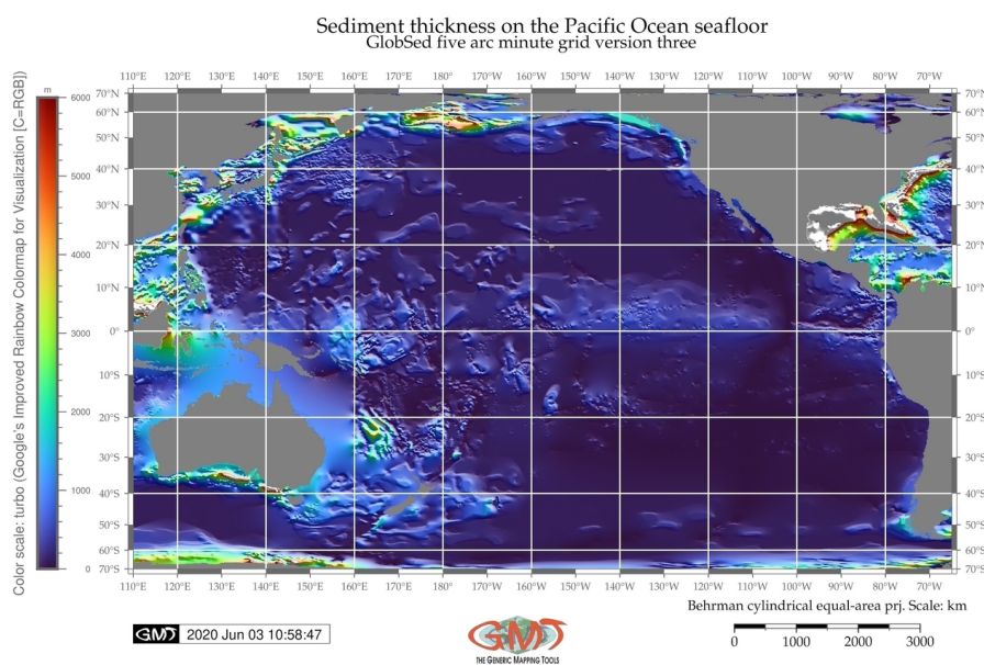
FIGURE 4 Sediment thickness of the Pacific Ocean seafloor. author
