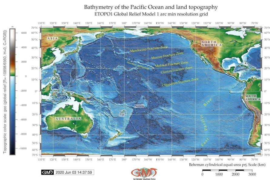
FIGURE 1 General bathymetric map of the Pacific Ocean. author
