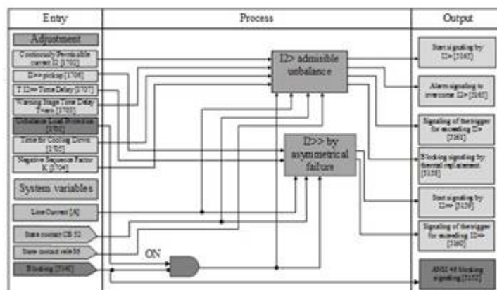
Figure 7 Confirmation sub-process ON ANSI 46 PDF 5
