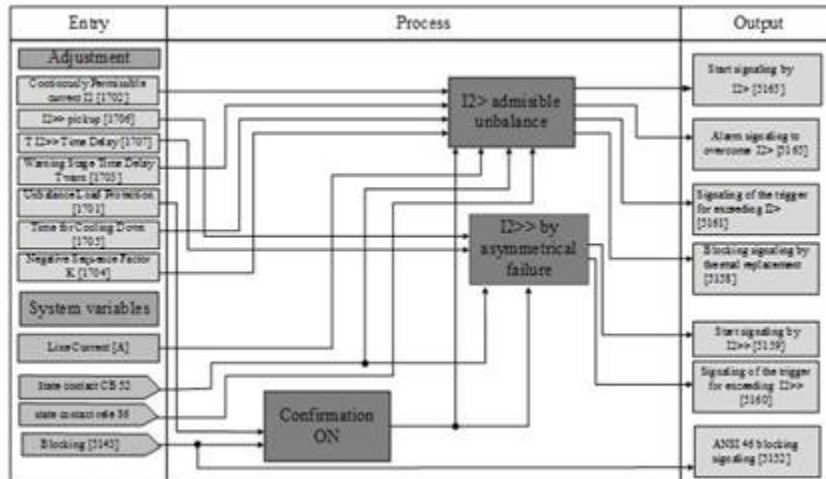
Figure 6 Complete logical diagram of ANSI 46 PDF (5).
