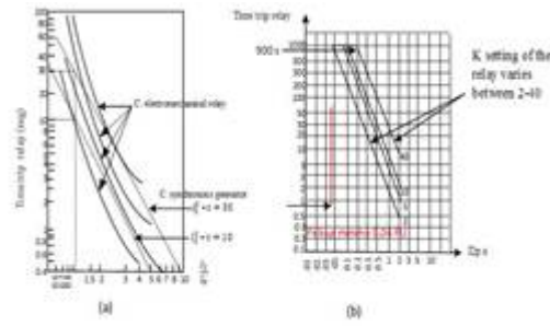
Figure 5 Operation characteristic of the PDF ANSI 46 of an electromechanical relay (a) and a digital relay (b). 2
