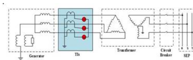
Figure 1 Connection of unbalanced load - negative sequence (ANSI 46 PDF)
