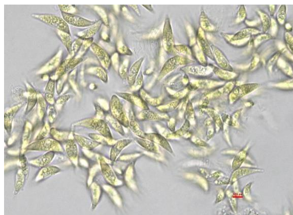
Figure 1. (b) Microscopic revision of monoalgal culture
