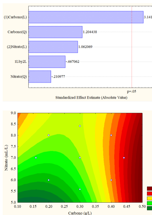
Figure 4b. Pareto diagram and surface response graphic for sodium carbonate/sodium nitrate
