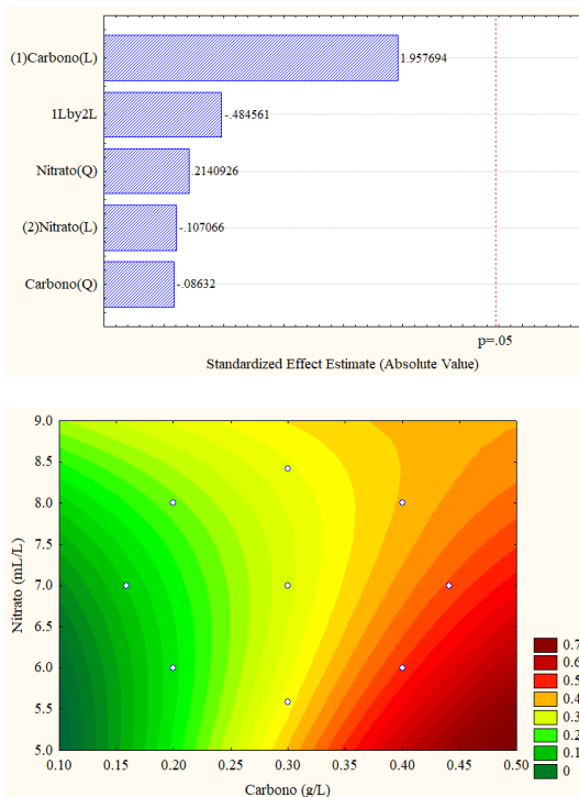
Figure 4c. Pareto diagram and surface response graphic for sodium bicarbonate/sodium nitrate
