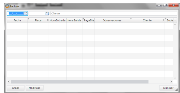
Figure 6. Billing Module
